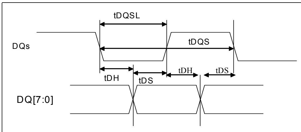
Figure 8-26. Dual Channel Interface Timings
